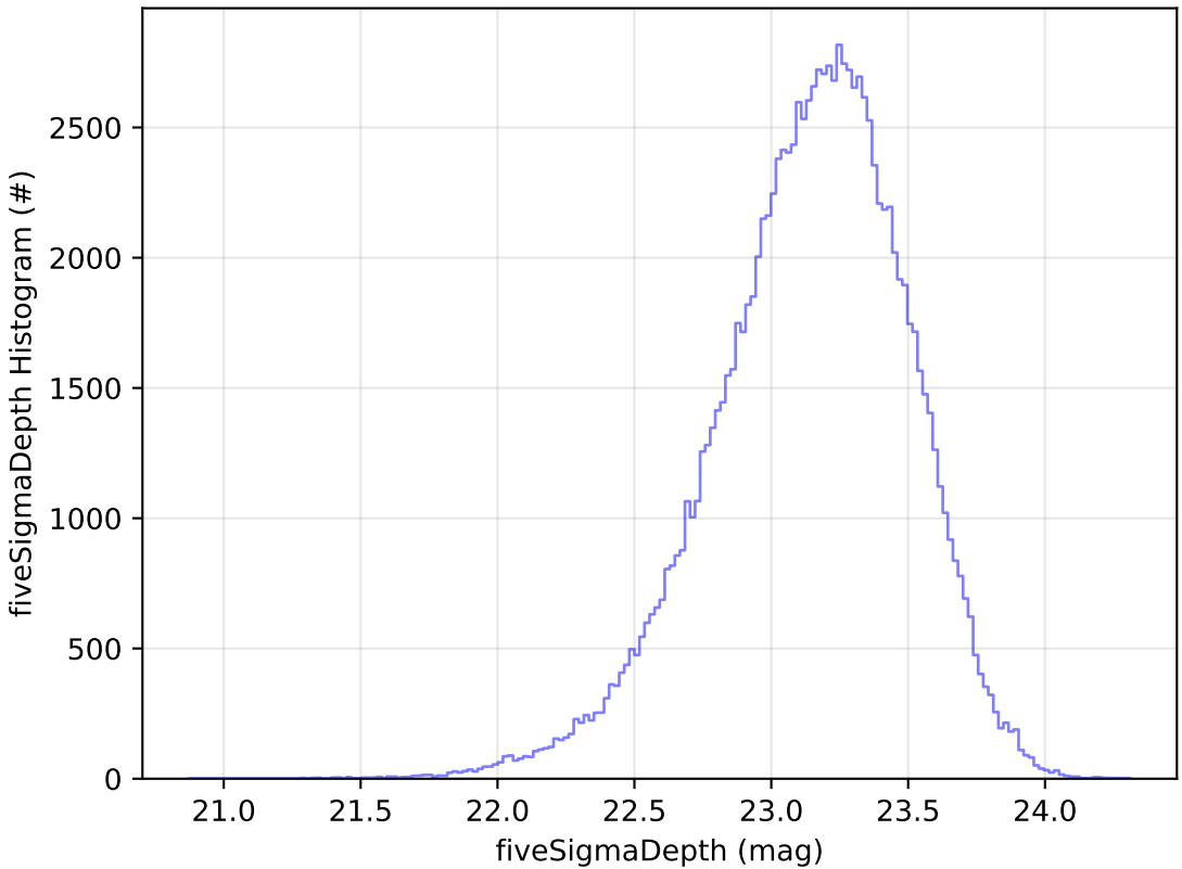
ddf_acor_sf25_lsf30_lsr20_v3.4_10yrs u: fiveSigmaDepth Histogram
