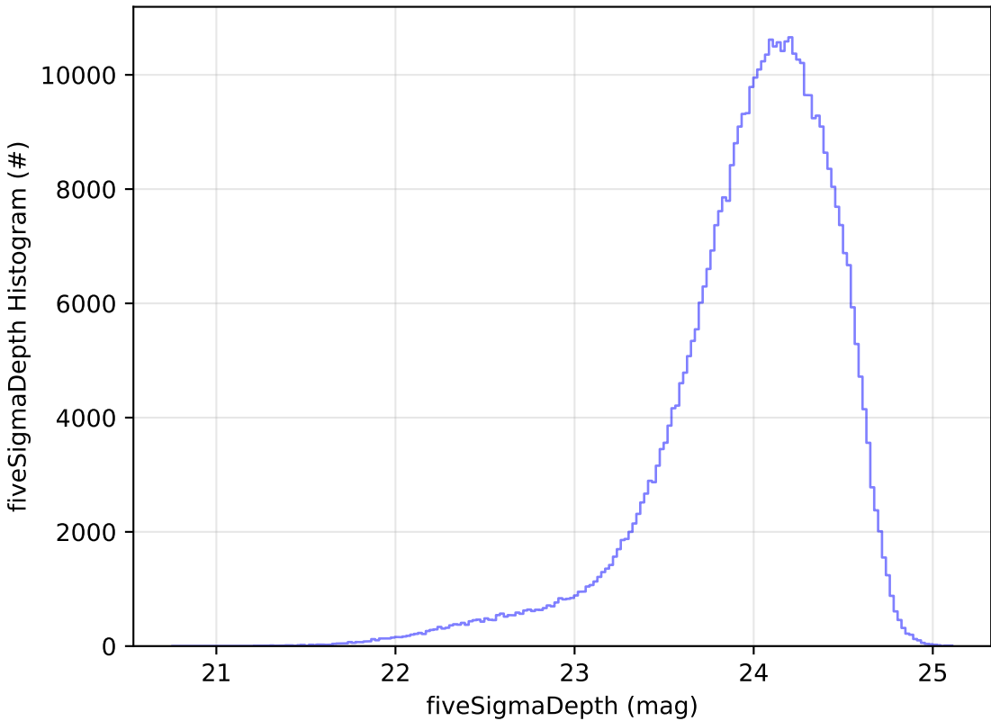
ddf_acor_sf25_lsf30_lsr20_v3.4_10yrs r: fiveSigmaDepth Histogram
