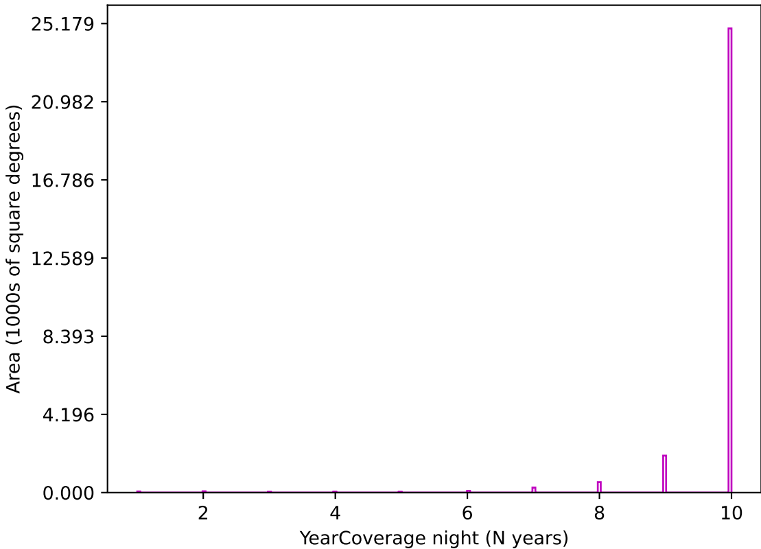
ddf_acor_sf25_lsf30_lsr20_v3.4_10yrs z band: YearCoverage night
