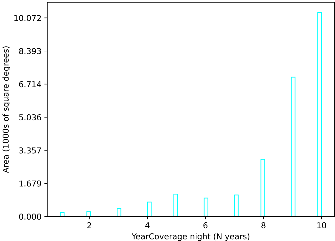
ddf_acor_sf25_lsf30_lsr20_v3.4_10yrs u band: YearCoverage night
