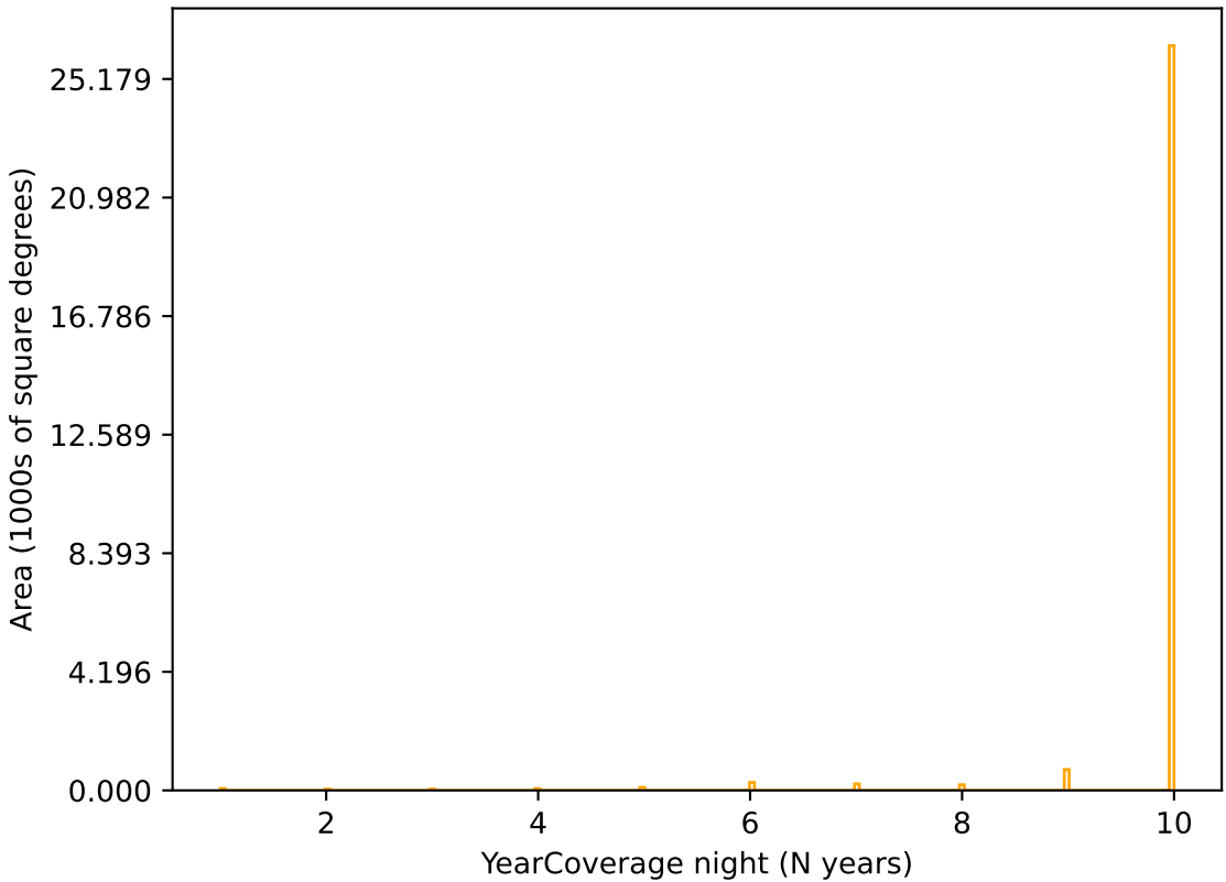
ddf_acor_sf25_lsf30_lsr20_v3.4_10yrs r band: YearCoverage night
