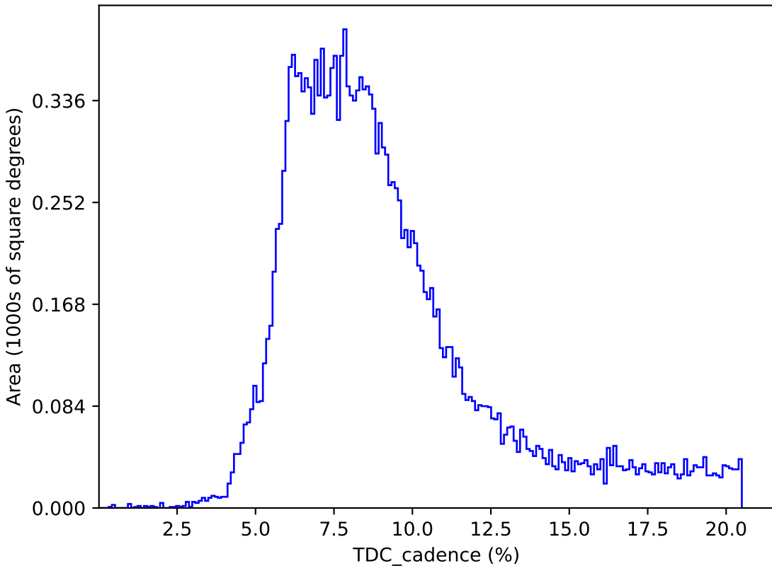
ddf_acor_sf25_ls30_lsr20_v3.4_10yrs : TDC_cadence
