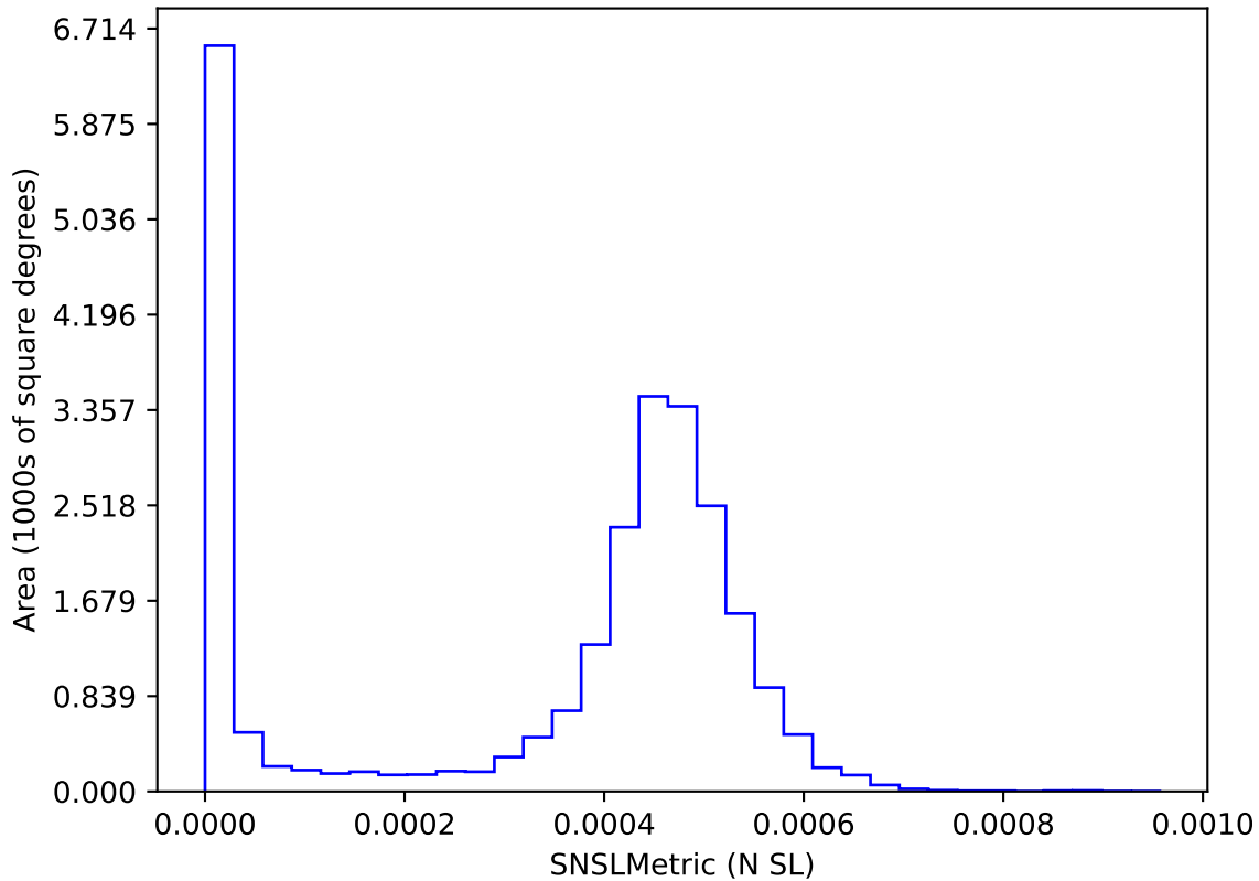
ddf_acor_sf25_lsf30_lsr20_v3.4_10yrs : SNSLMetric
