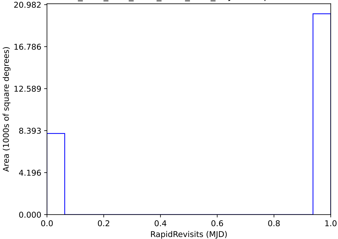
ddf_acor_sf25_lsf30_lsr20_v3.4_10yrs : RapidRevisits
