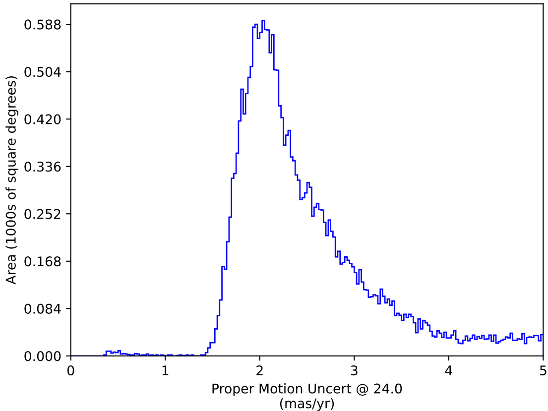
ddf_acor_sf25_lsf30_lsr20_v3.4_10yrs : Proper Motion Uncert @ 24.0
