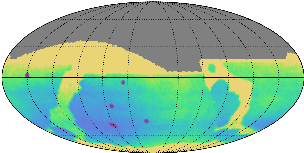
ddf_acor_sf25_lsf30_lsr20_v3.4_10yrs : Parallax Uncert @ 24.0
