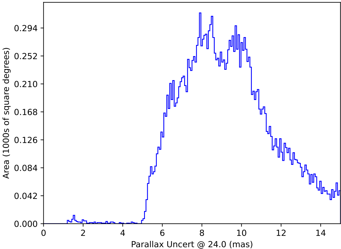
ddf_acor_sf25_lsf30_lsr20_v3.4_10yrs : Parallax Uncert @ 24.0
