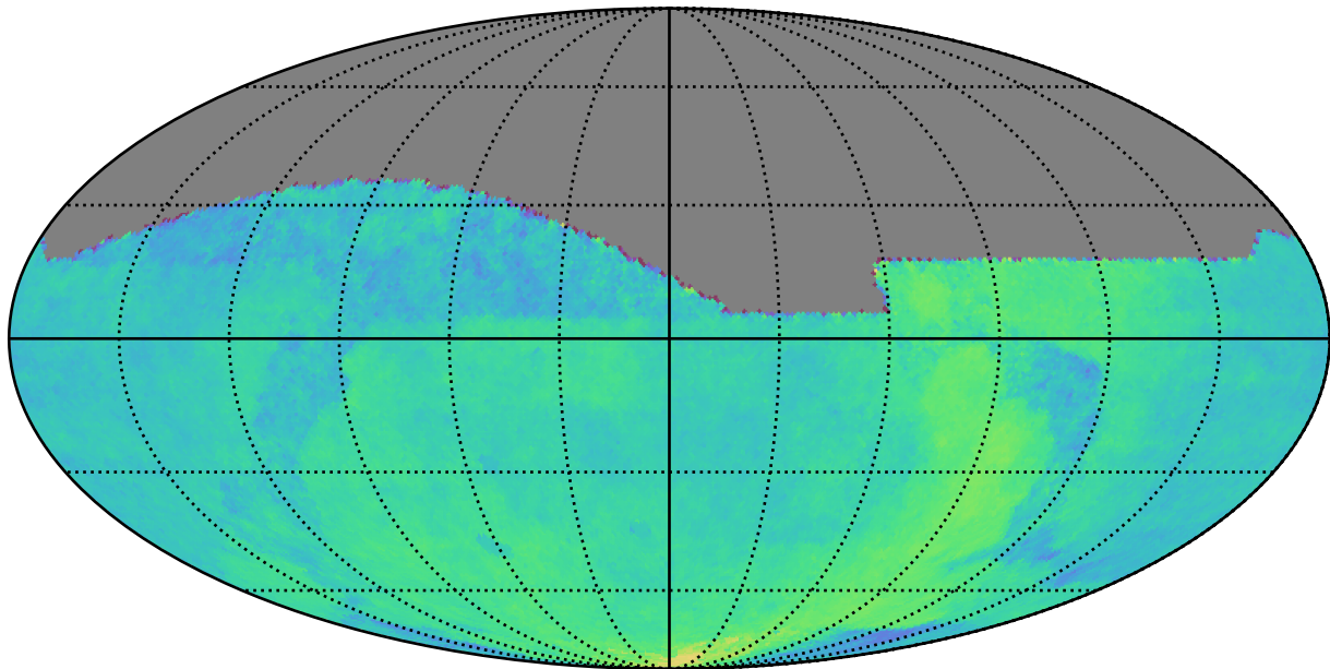
ddf_acor_sf25_lsf30_lsr20_v3.4_10yrs : Parallax Coverage @ 22.4
