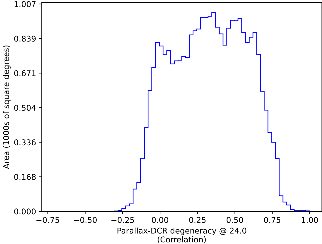
ddf_acor_sf25_lsf30_lsr20_v3.4_10yrs : Parallax-DCR degeneracy @ 24.0
