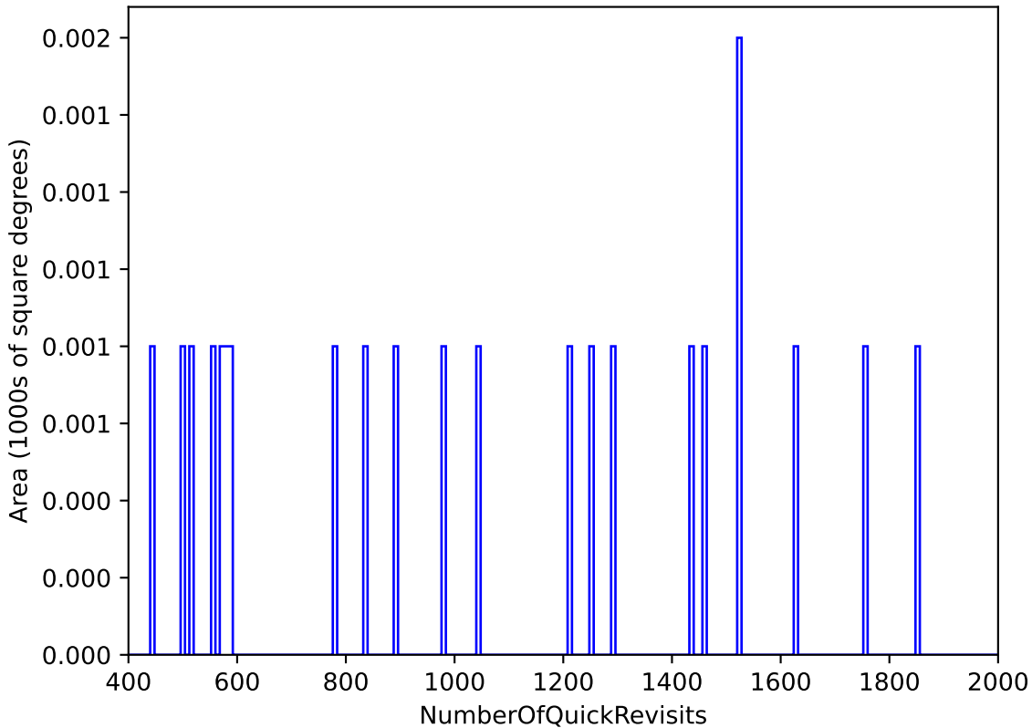
ddf_acor_sf25_lsf30_lsr20_v3.4_10yrs : NumberOfQuickRevisits
