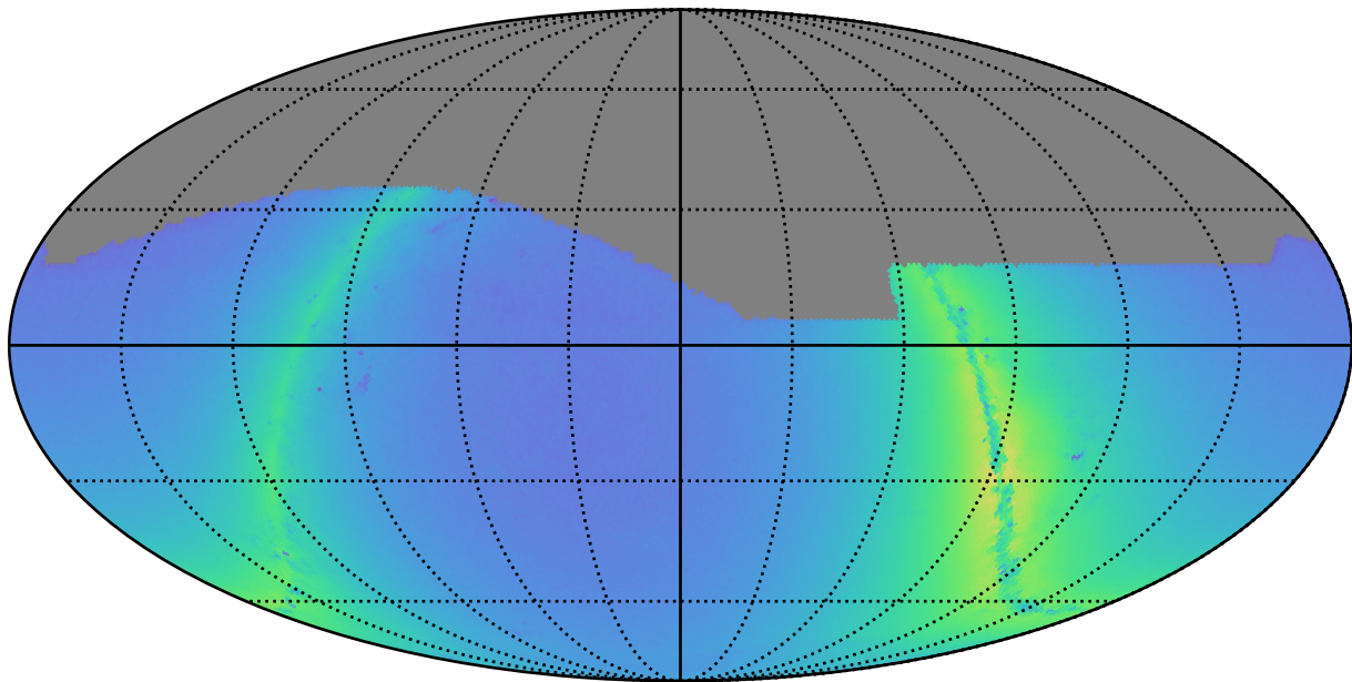
ddf_acor_sf25_lsf30_lsr20_v3.4_10yrs r: Nstars_no_crowding
