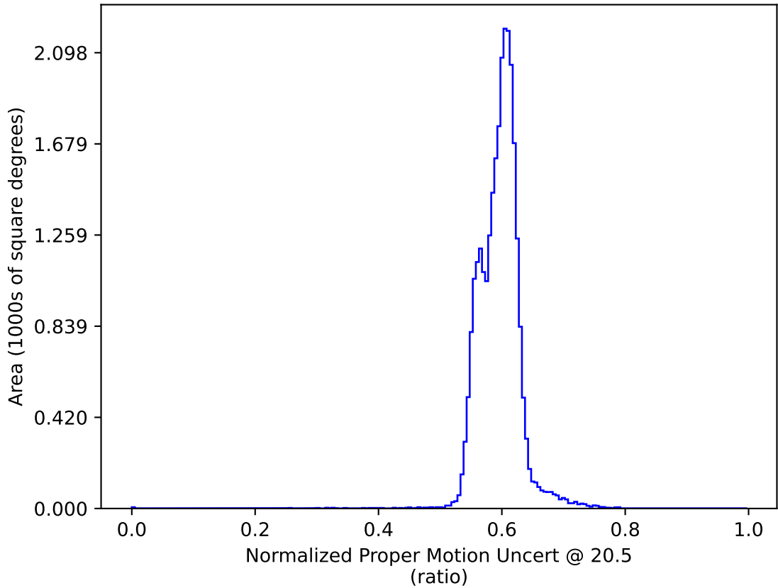
ddf_acor_sf25_lsf30_lsr20_v3.4_10yrs : Normalized Proper Motion Uncert @ 20.5
