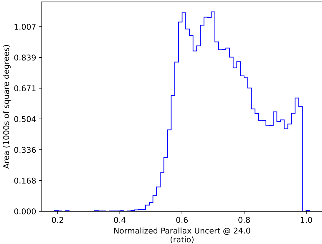
ddf_acor_sf25_lsf30_lsr20_v3.4_10yrs : Normalized Parallax Uncert @ 24.0
