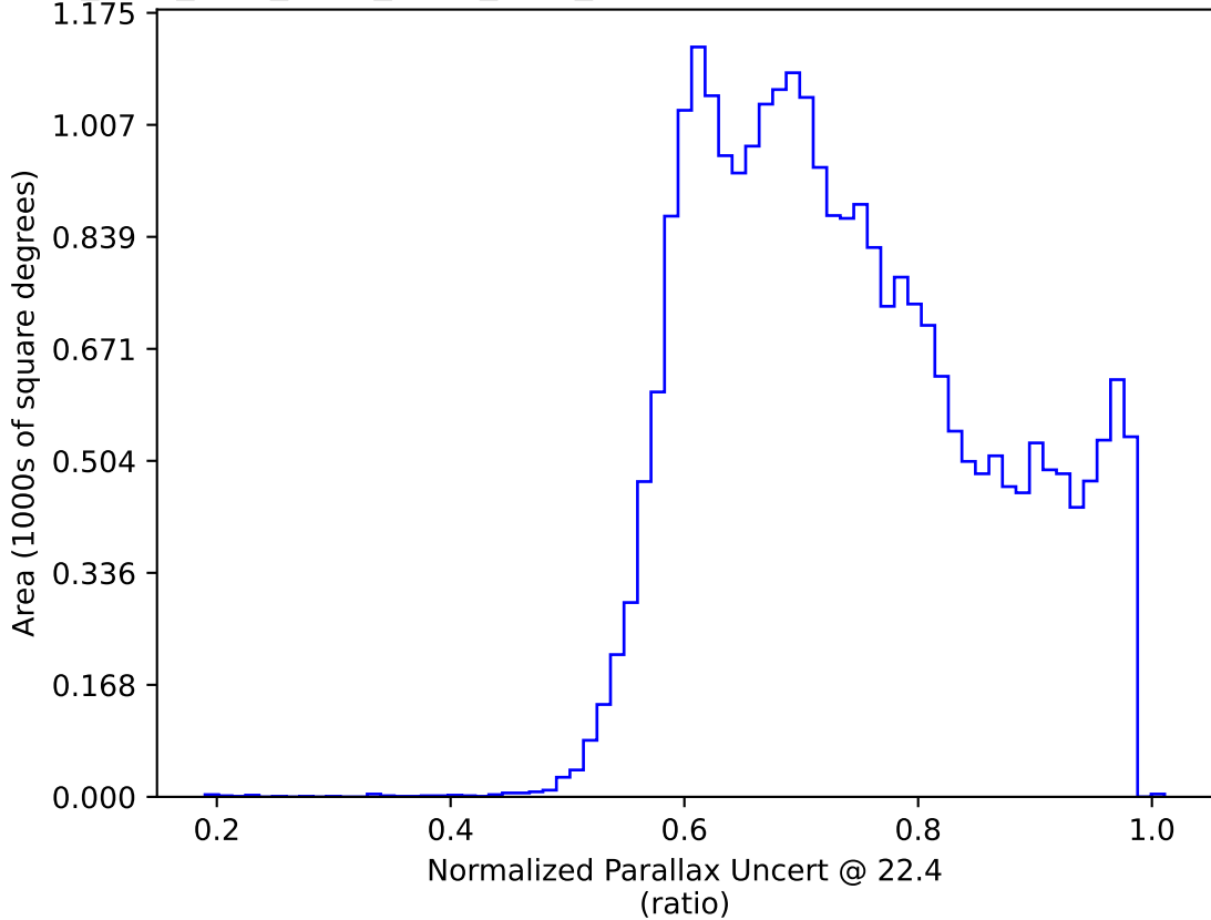
ddf_acor_sf25_lsf30_lsr20_v3.4_10yrs : Normalized Parallax Uncert @ 22.4
