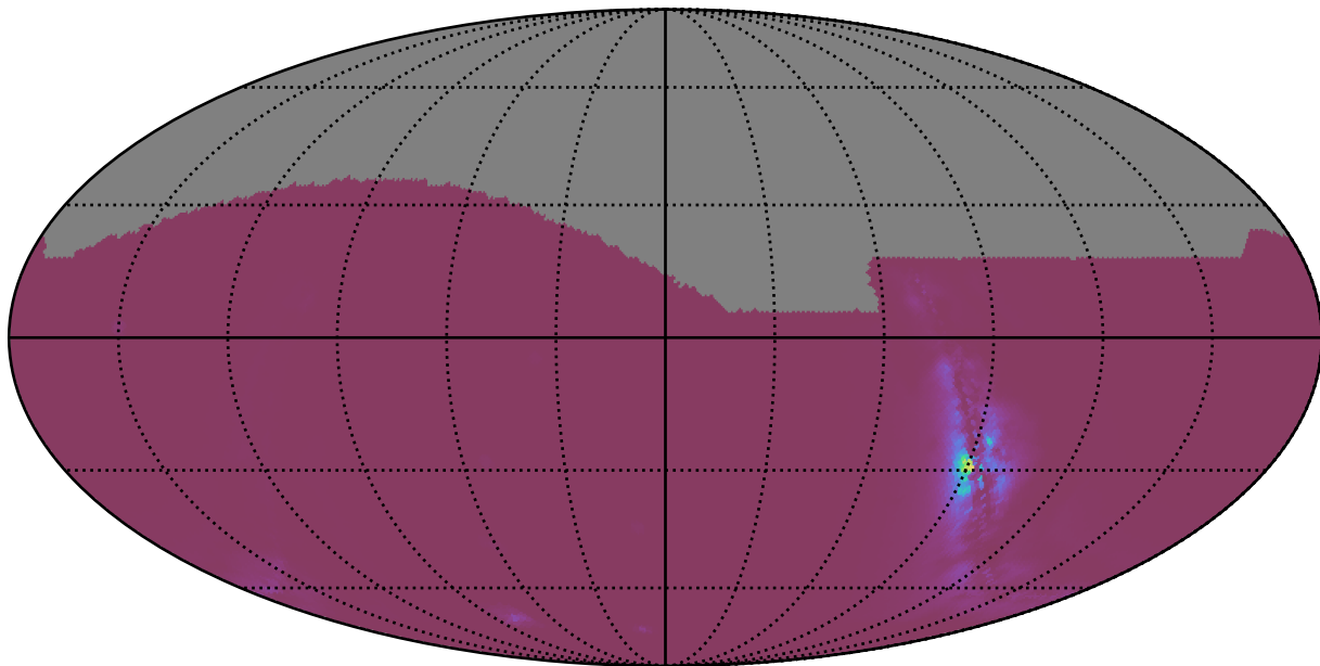
ddf_acor_sf25_lsf30_lsr20_v3.4_10yrs : NlcPoints
