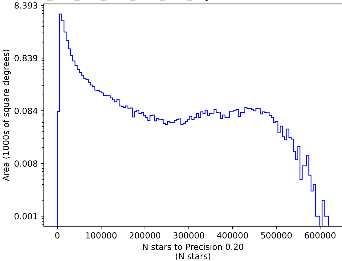
ddf_acor_sf25_lsf30_lsr20_v3.4_10yrs i: N stars to Precision 0.20
