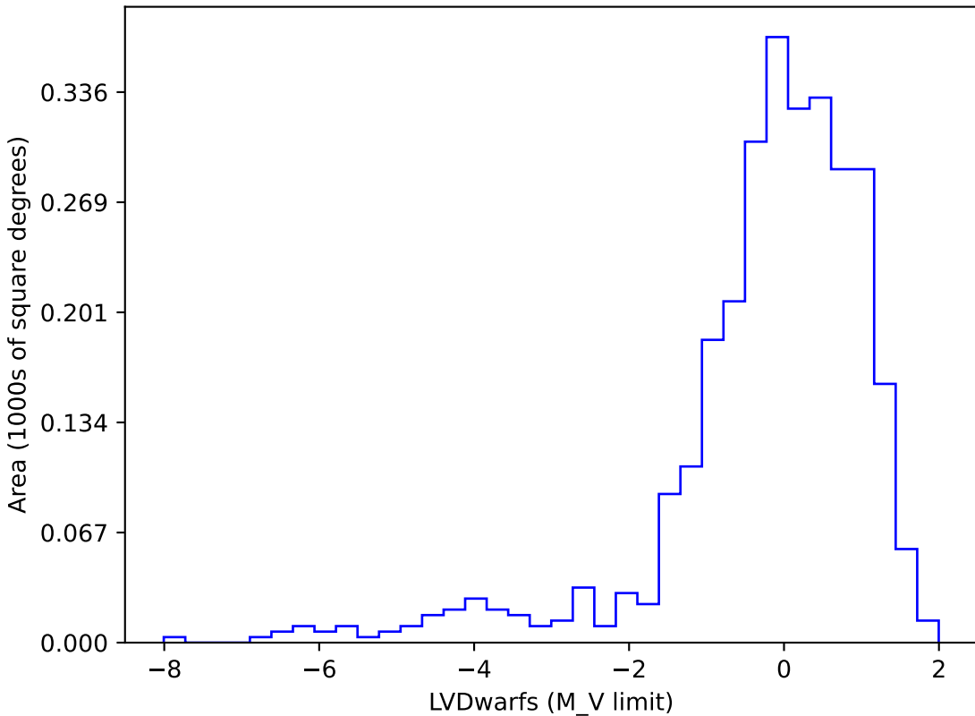
ddf_acor_sf25_lsf30_lsr20_v3.4_10yrs gi SCP: LVDwarfs
