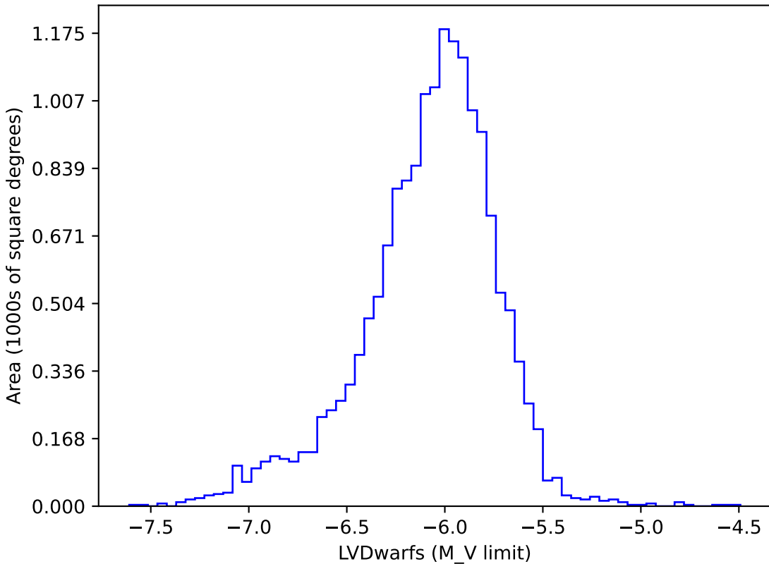
ddf_acor_sf25_lsf30_lsr20_v3.4_10yrs gi: LVDwarfs
