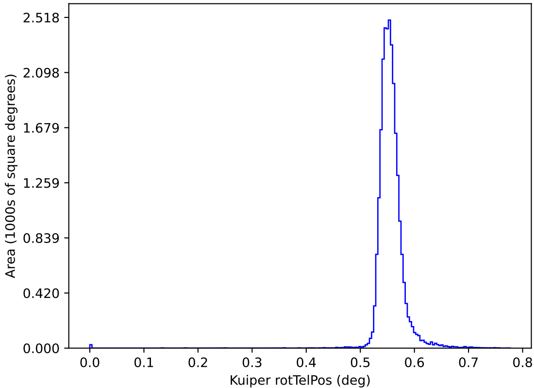
ddf_acor_sf25_lsf30_lsr20_v3.4_10yrs y: Kuiper rotTelPos
