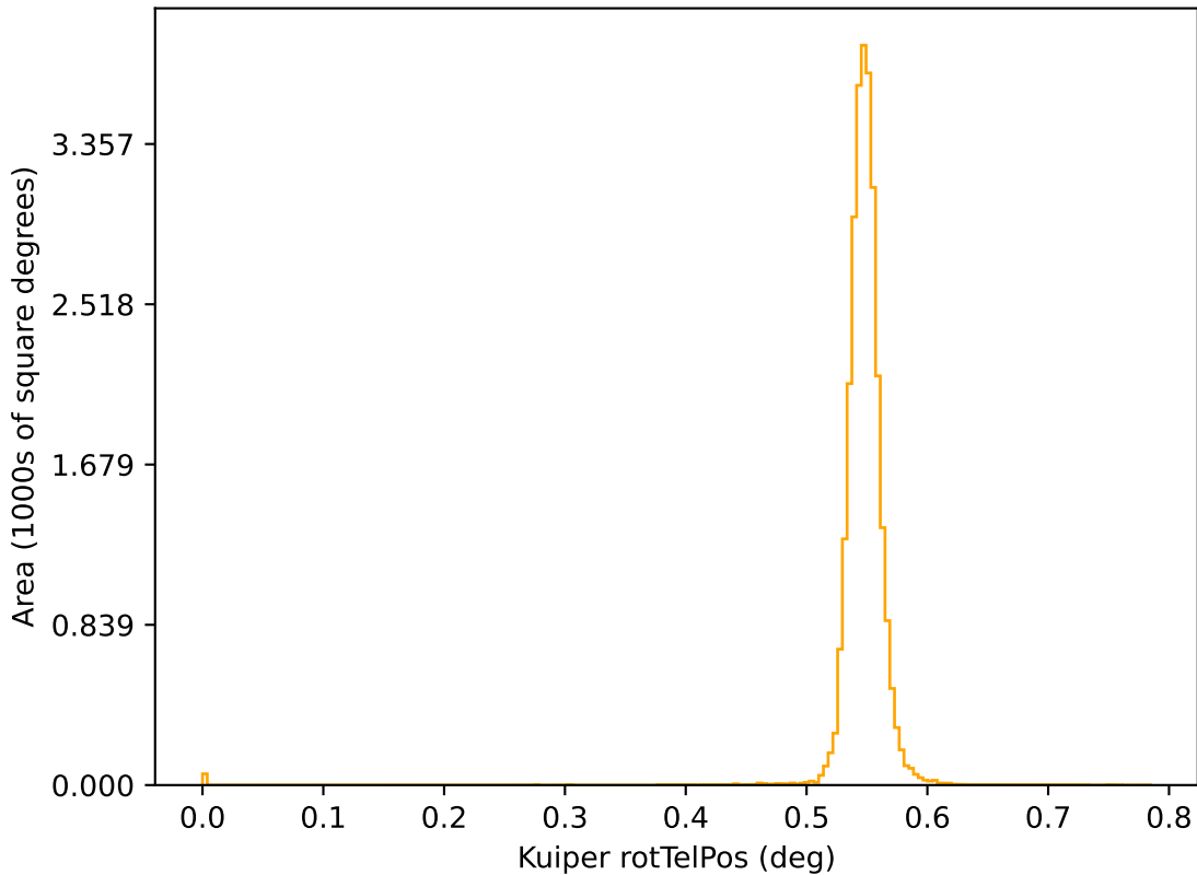
ddf_acor_sf25_lsf30_lsr20_v3.4_10yrs r: Kuiper rotTelPos
