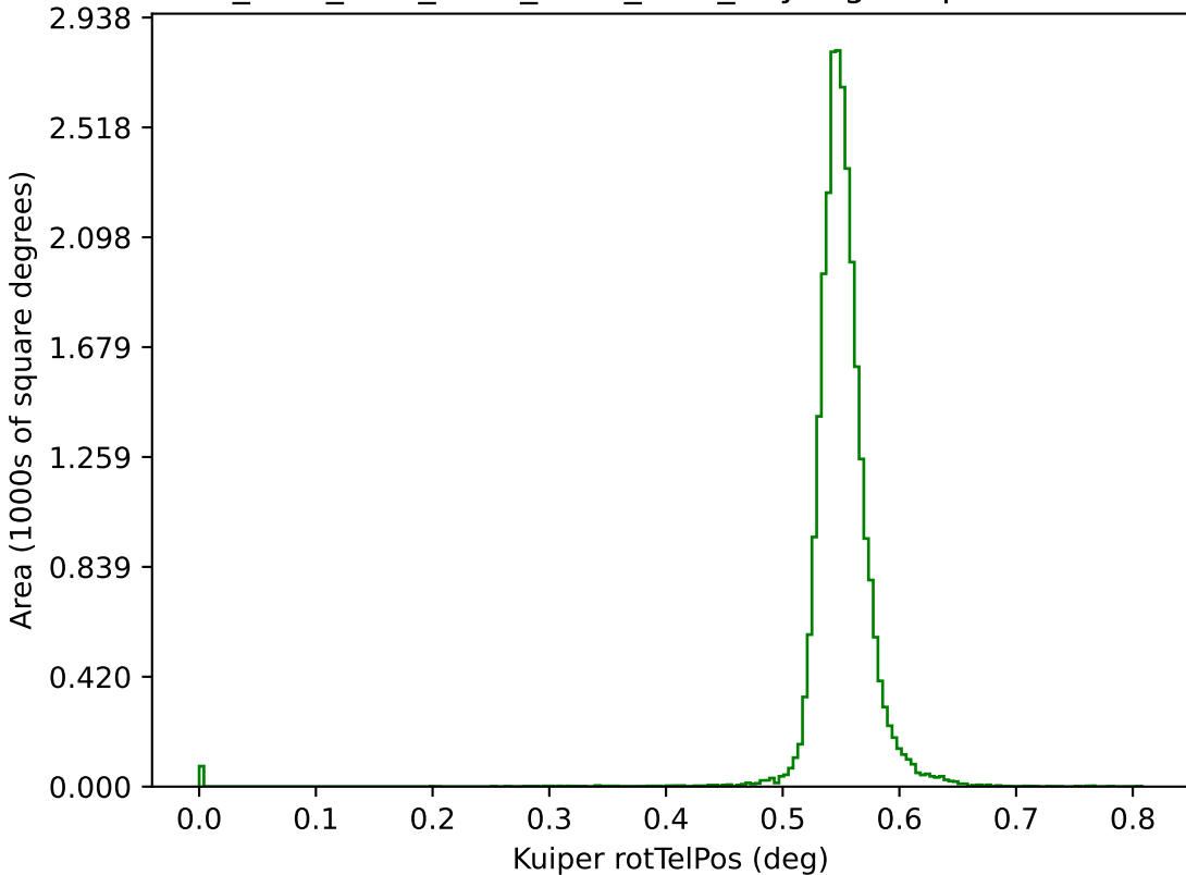
ddf_acor_sf25_lsf30_lsr20_v3.4_10yrs g: Kuiper rotTelPos
