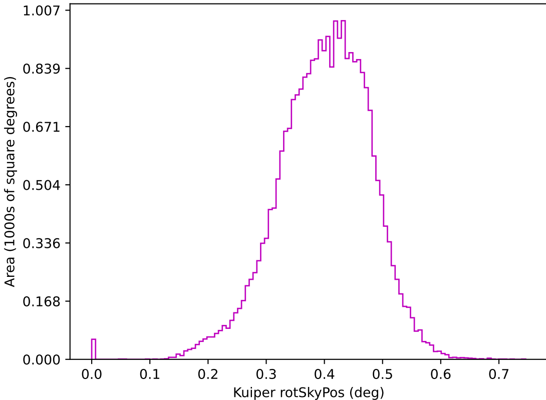
ddf_acor_sf25_lsf30_lsr20_v3.4_10yrs z: Kuiper rotSkyPos
