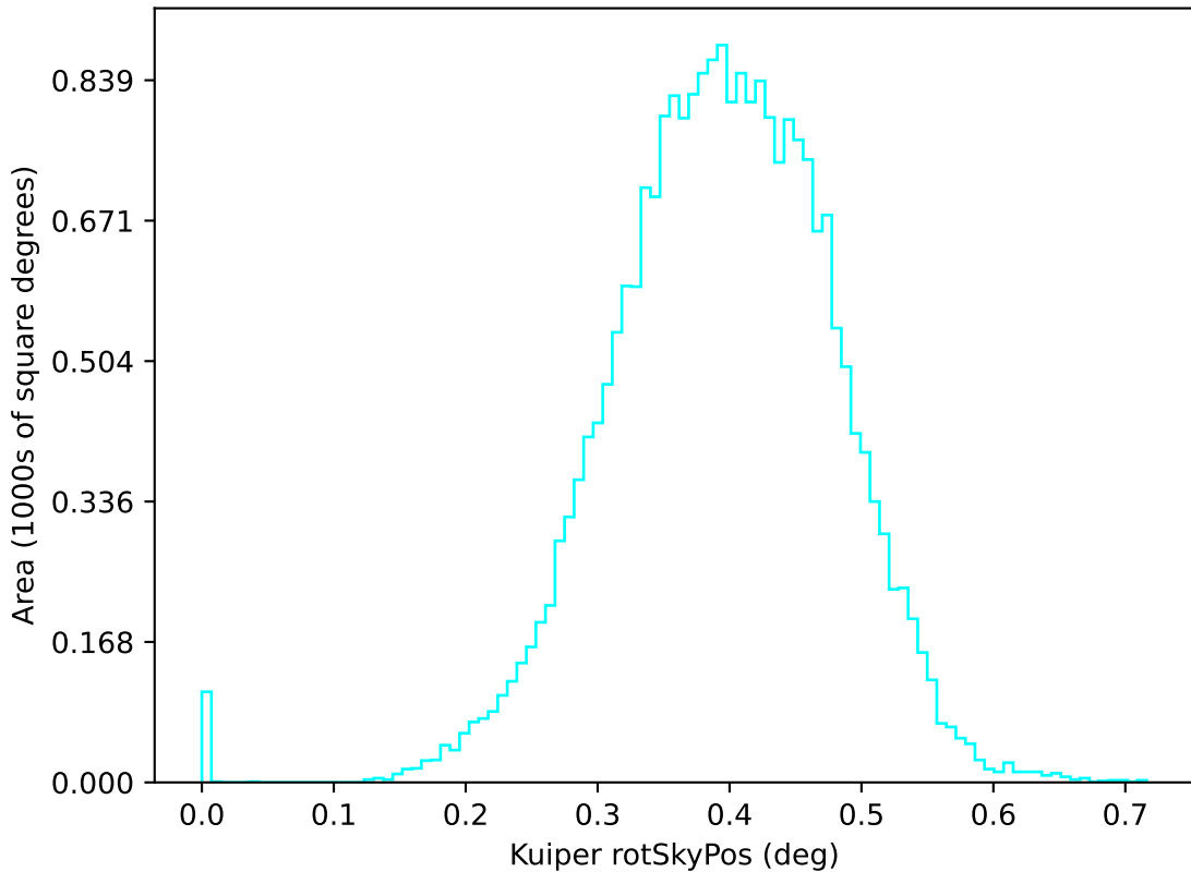
ddf_acor_sf25_lsf30_lsr20_v3.4_10yrs u: Kuiper rotSkyPos
