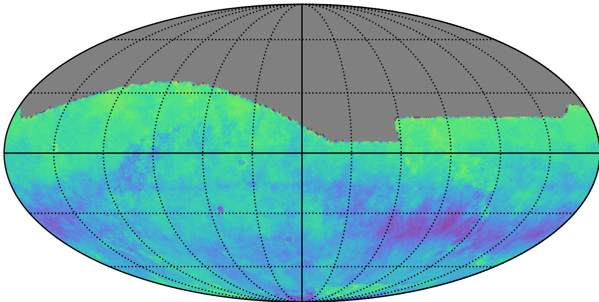
ddf_acor_sf25_lsf30_lsr20_v3.4_10yrs r: Kuiper rotSkyPos
