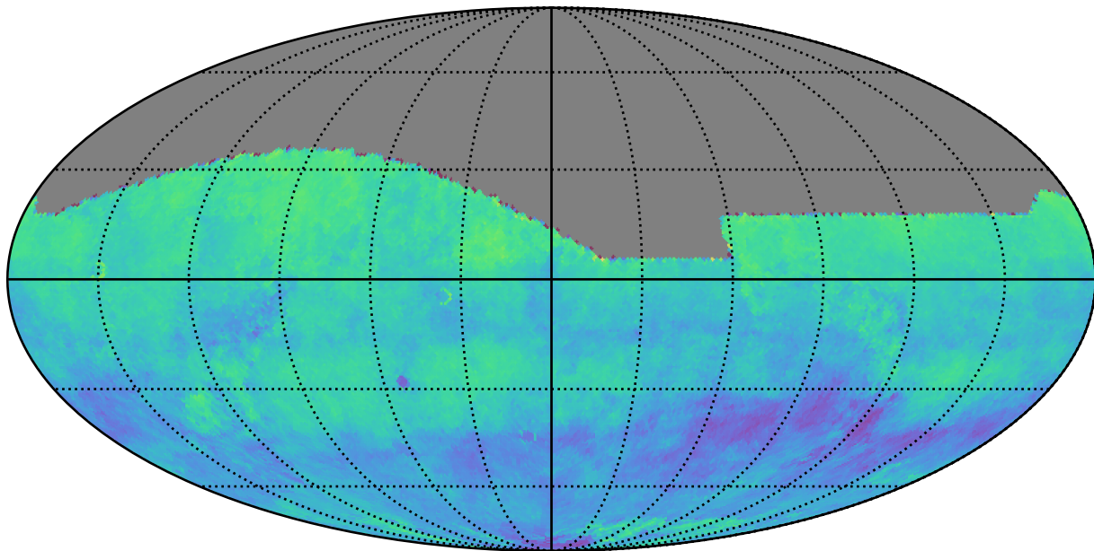
ddf_acor_sf25_lsf30_lsr20_v3.4_10yrs i: Kuiper rotSkyPos
