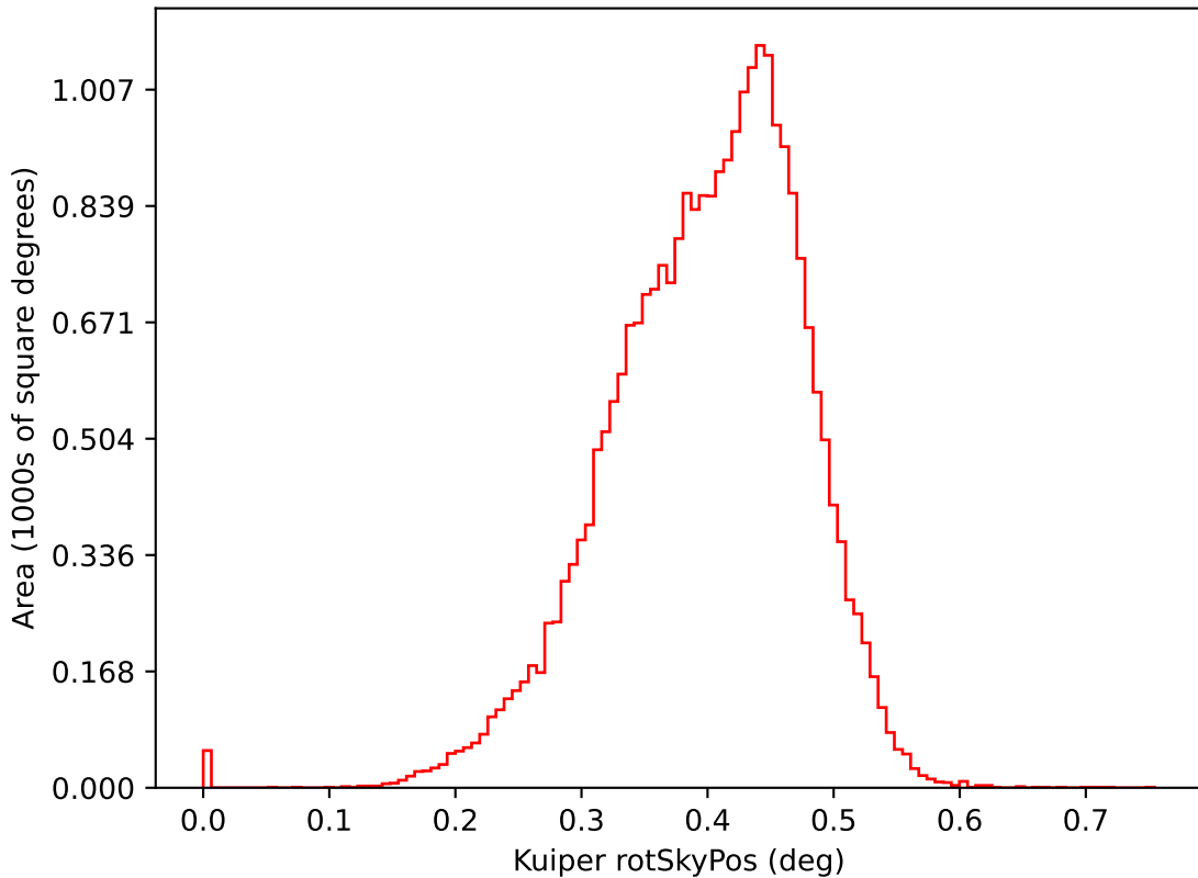
ddf_acor_sf25_lsf30_lsr20_v3.4_10yrs i: Kuiper rotSkyPos
