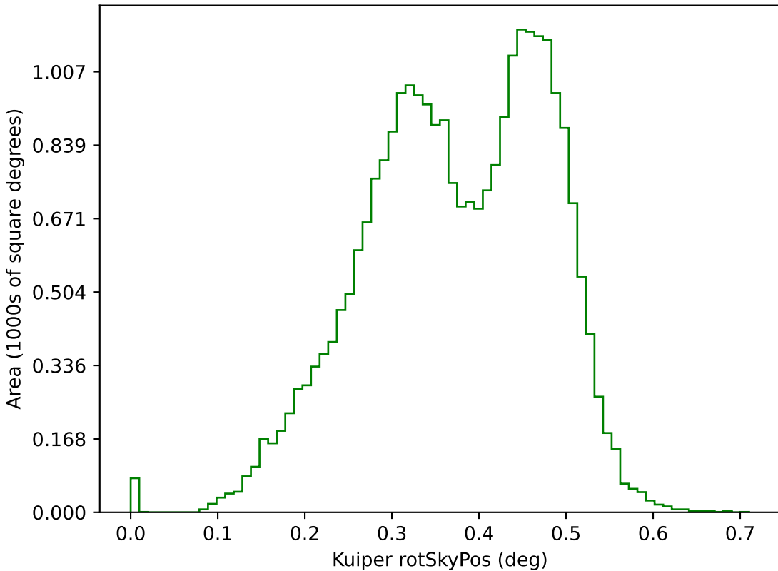
ddf_acor_sf25_lsf30_lsr20_v3.4_10yrs g: Kuiper rotSkyPos
