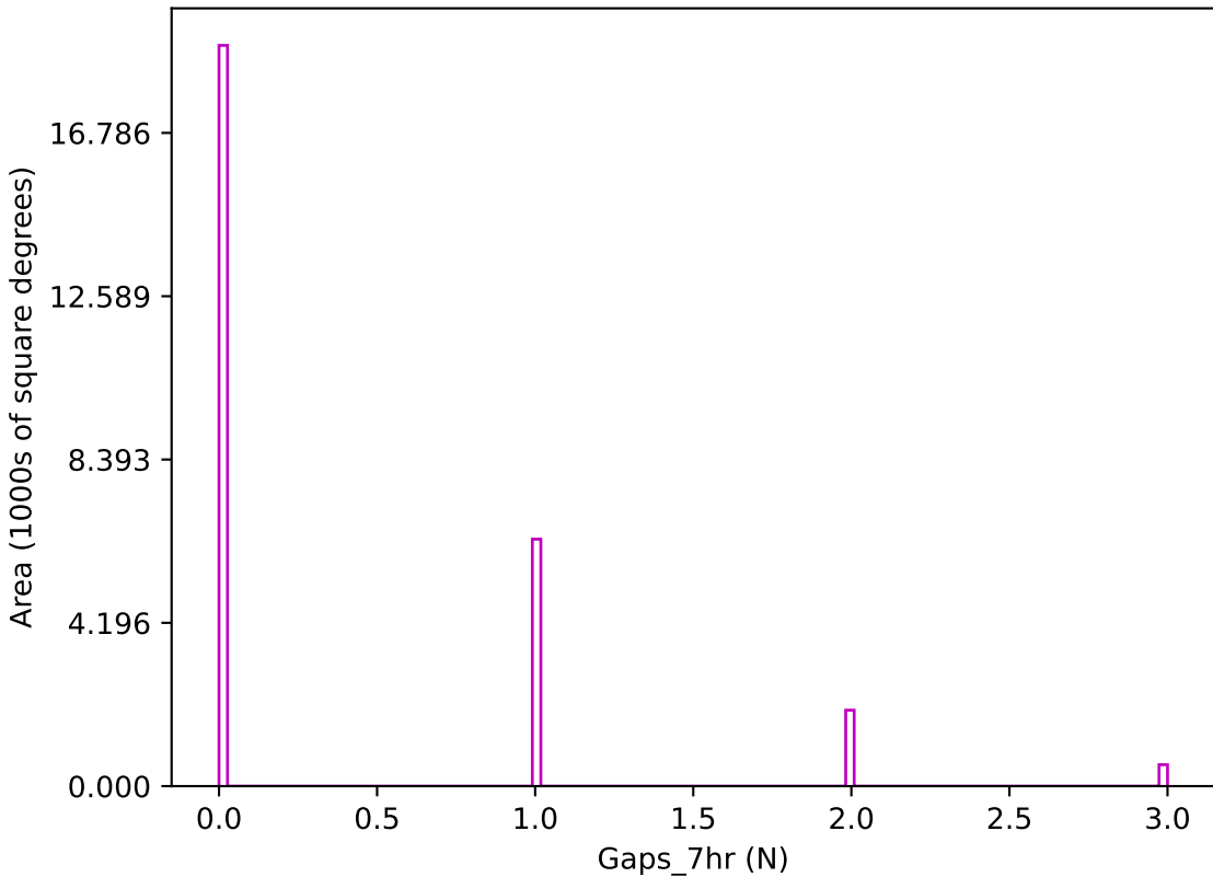
ddf_acor_sf25_ls30_lsr20_v3.4_10yrs z band: Gaps_7hr
