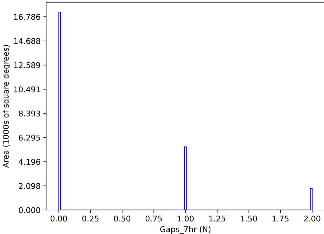
ddf_acor_sf25_ls30_lsr20_v3.4_10yrs y band: Gaps_7hr
