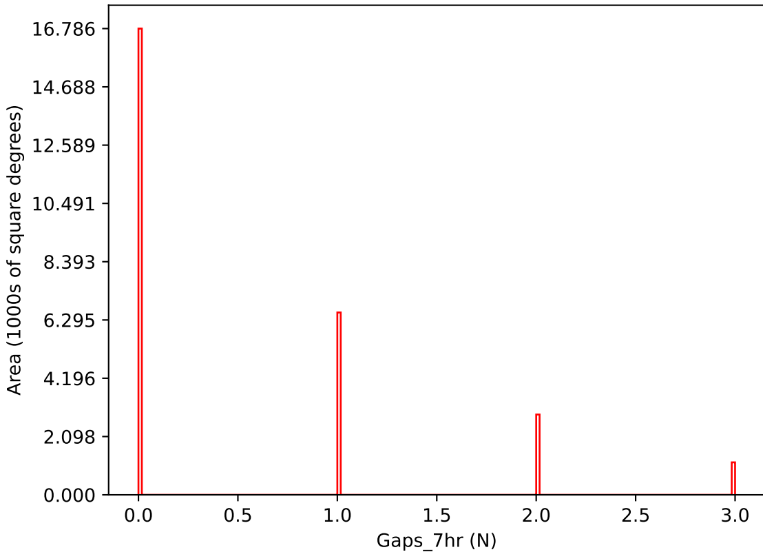
ddf_acor_sf25_lsf30_lsr20_v3.4_10yrs i band: Gaps_7hr
