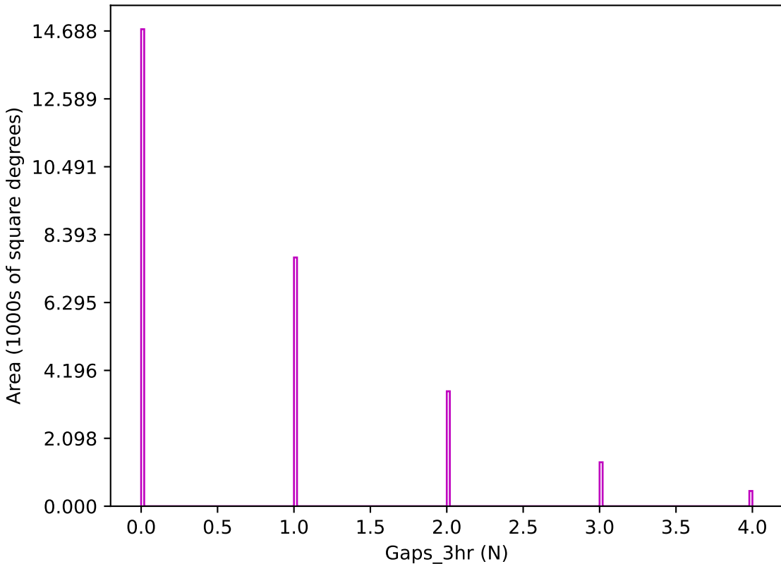
ddf_acor_sf25_lsf30_lsr20_v3.4_10yrs z band: Gaps_3hr
