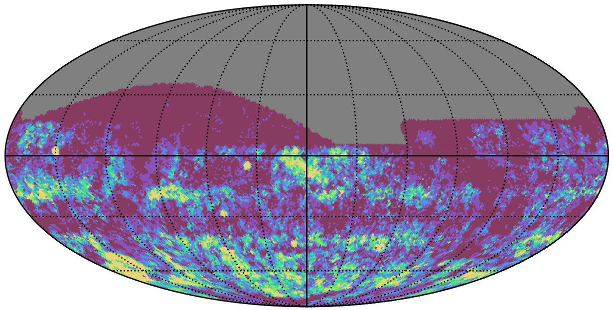
ddf_acor_sf25_lsf30_lsr20_v3.4_10yrs r band: Gaps_3hr
