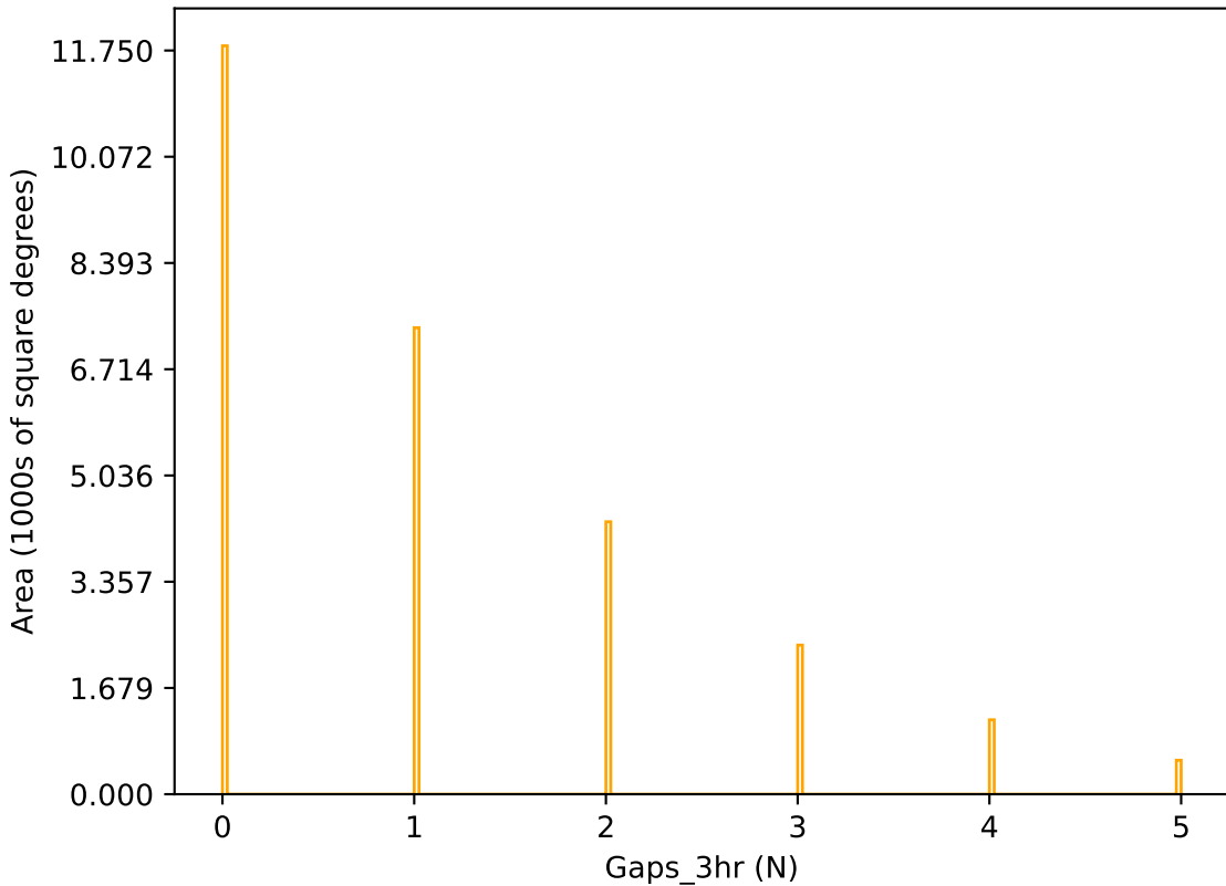
ddf_acor_sf25_lsf30_lsr20_v3.4_10yrs r band: Gaps_3hr
