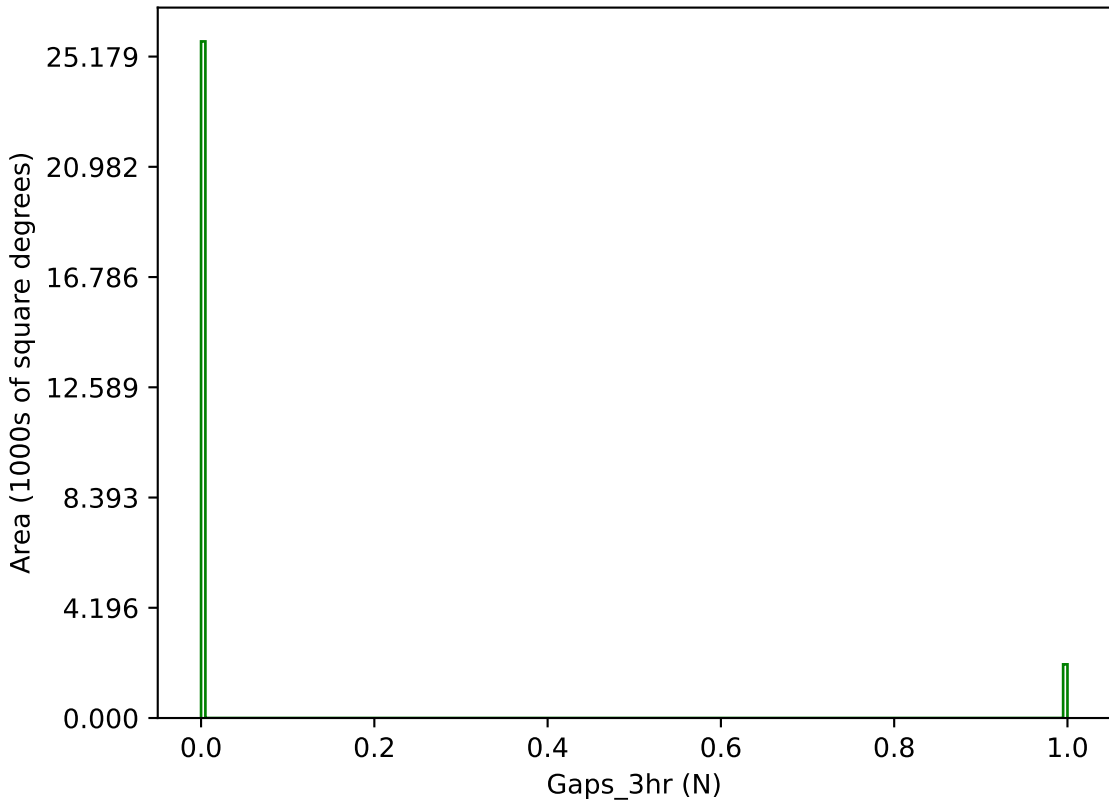
ddf_acor_sf25_lsf30_lsr20_v3.4_10yrs g band: Gaps_3hr
