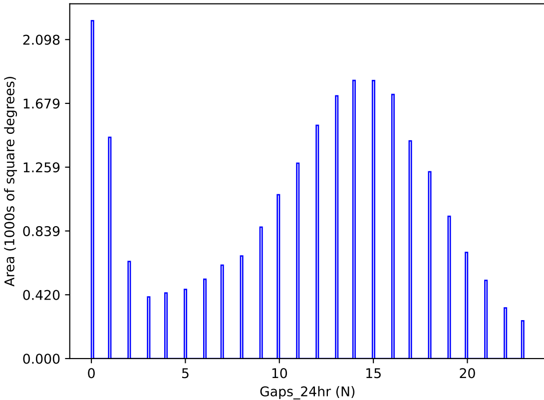
ddf_acor_sf25_lsf30_lsr20_v3.4_10yrs y band: Gaps_24hr
