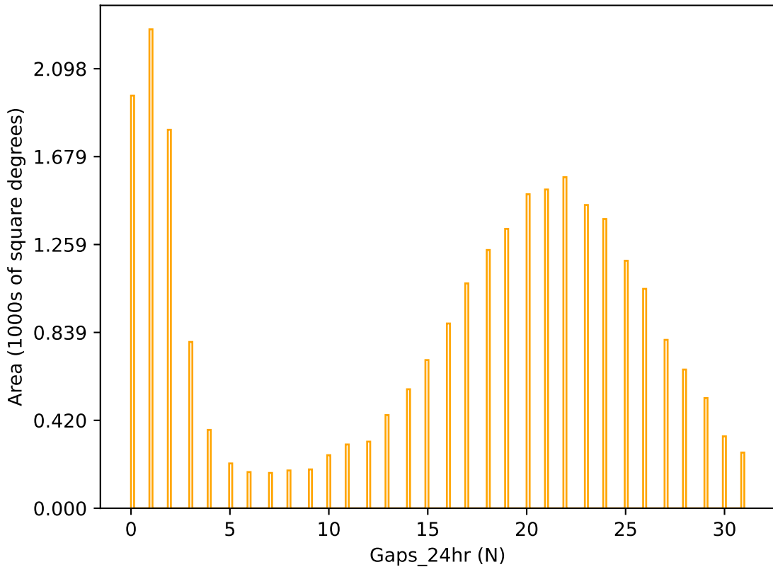
ddf_acor_sf25_lsf30_lsr20_v3.4_10yrs r band: Gaps_24hr
