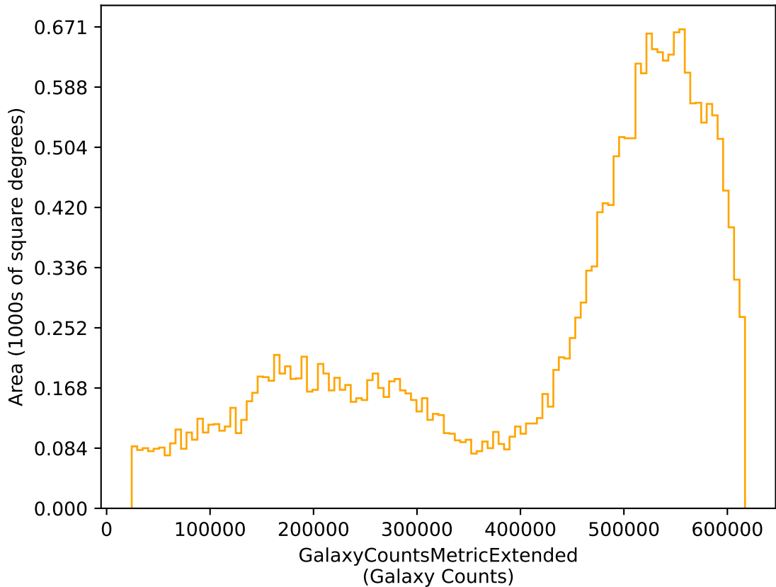
ddf_acor_sf25_lsf30_lsr20_v3.4_10yrs r: GalaxyCountsMetricExtended
