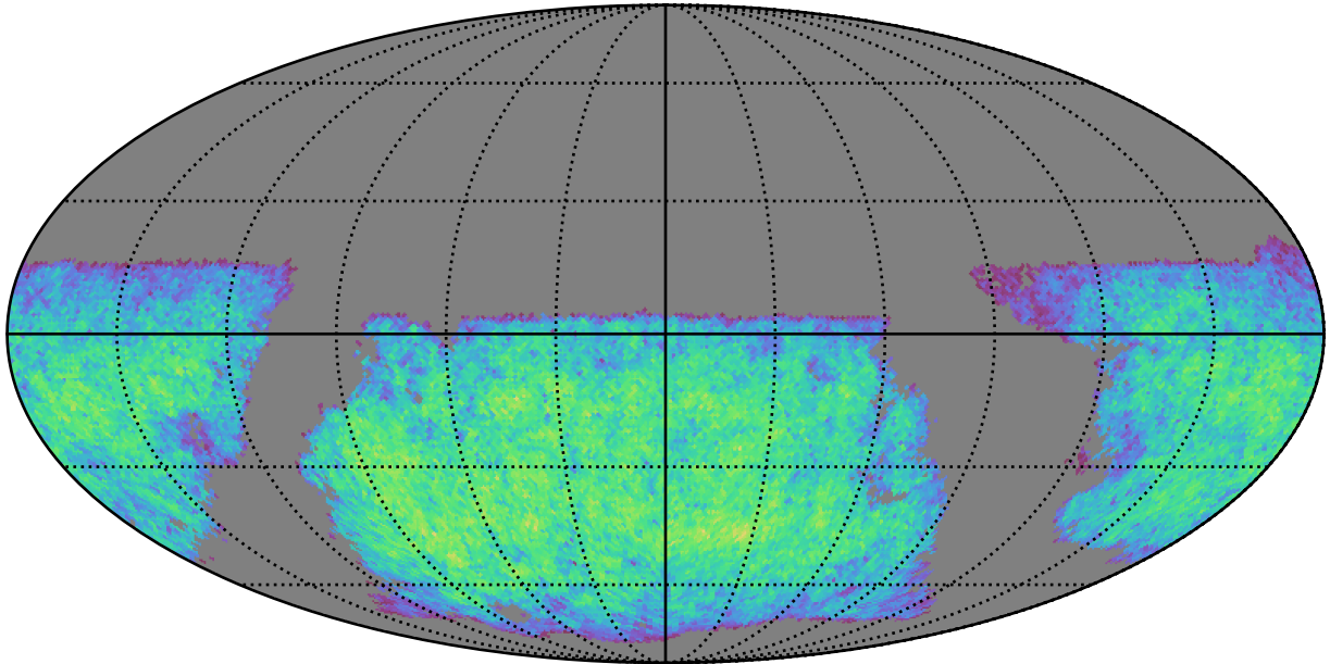
ddf_acor_sf25_lsf30_lsr20_v3.4_10yrs i band non-DD year 1: ExgalM5WithCuts
