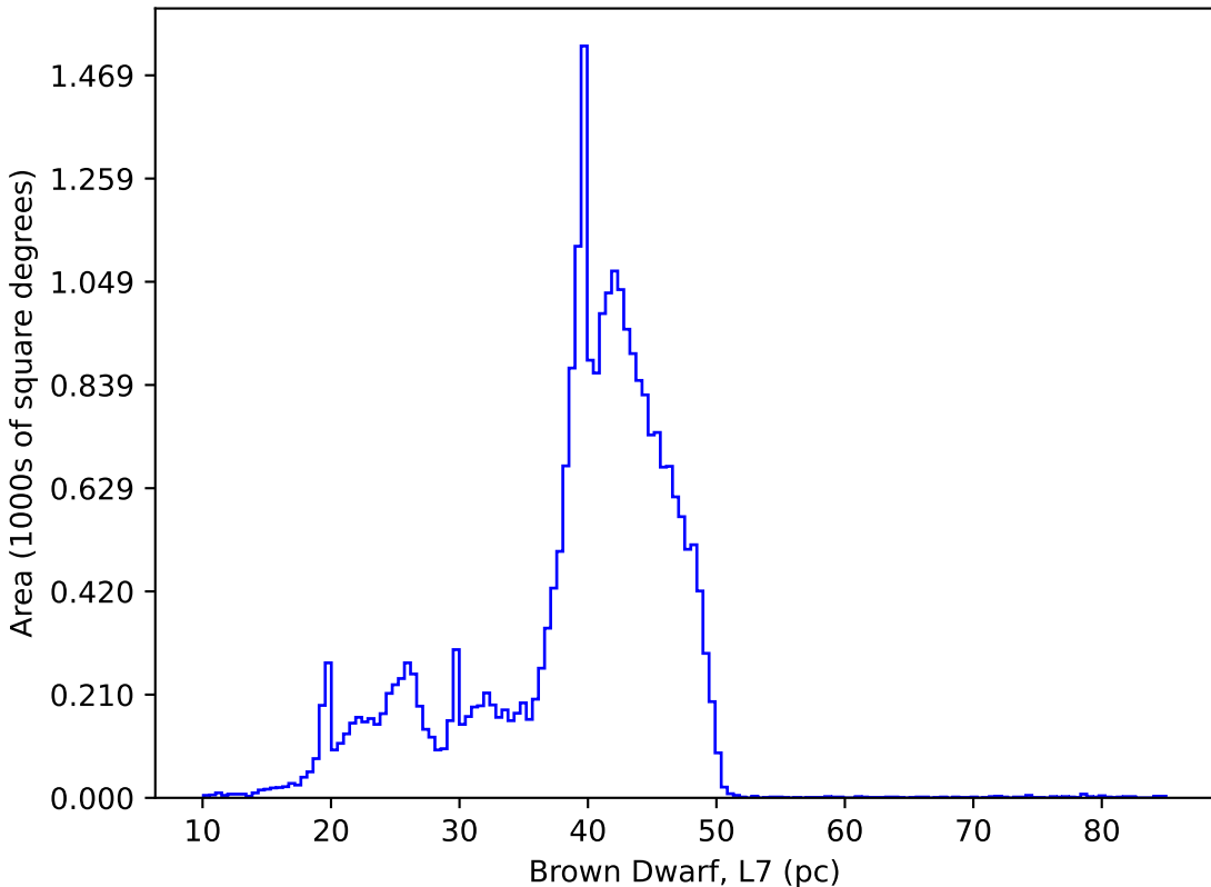
ddf_acor_sf25_lsf30_lsr20_v3.4_10yrs : Brown Dwarf, L7
