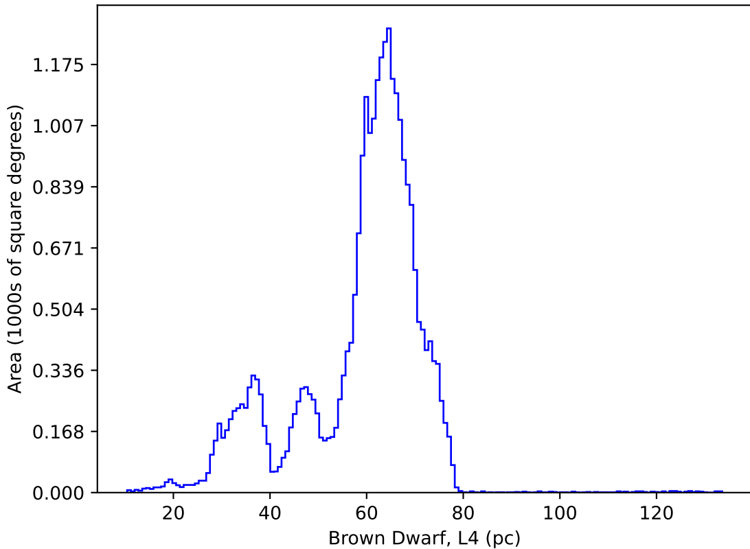
ddf_acor_sf25_lsf30_lsr20_v3.4_10yrs : Brown Dwarf, L4
