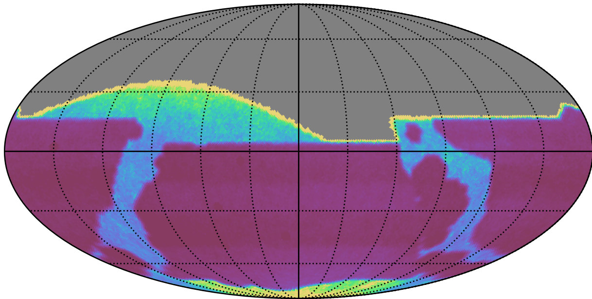
ddf_acor_sf25_lsf30_lsr20_v3.4_10yrs : properMotion
