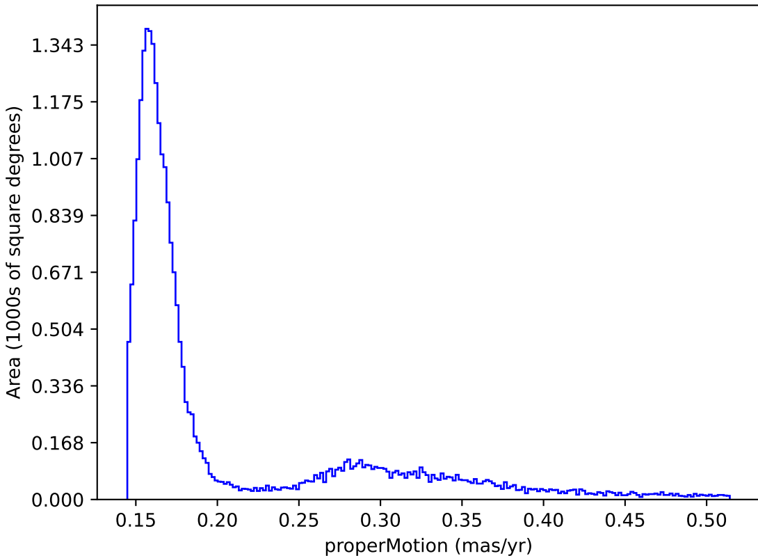
ddf_acor_sf25_lsf30_lsr20_v3.4_10yrs : properMotion
