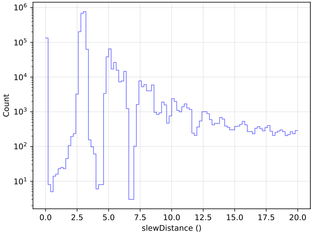
ddf_acor_sf25_lsf30_lsr20_v3.4_10yrs All visits: Zoom Slew Distance Histogram
