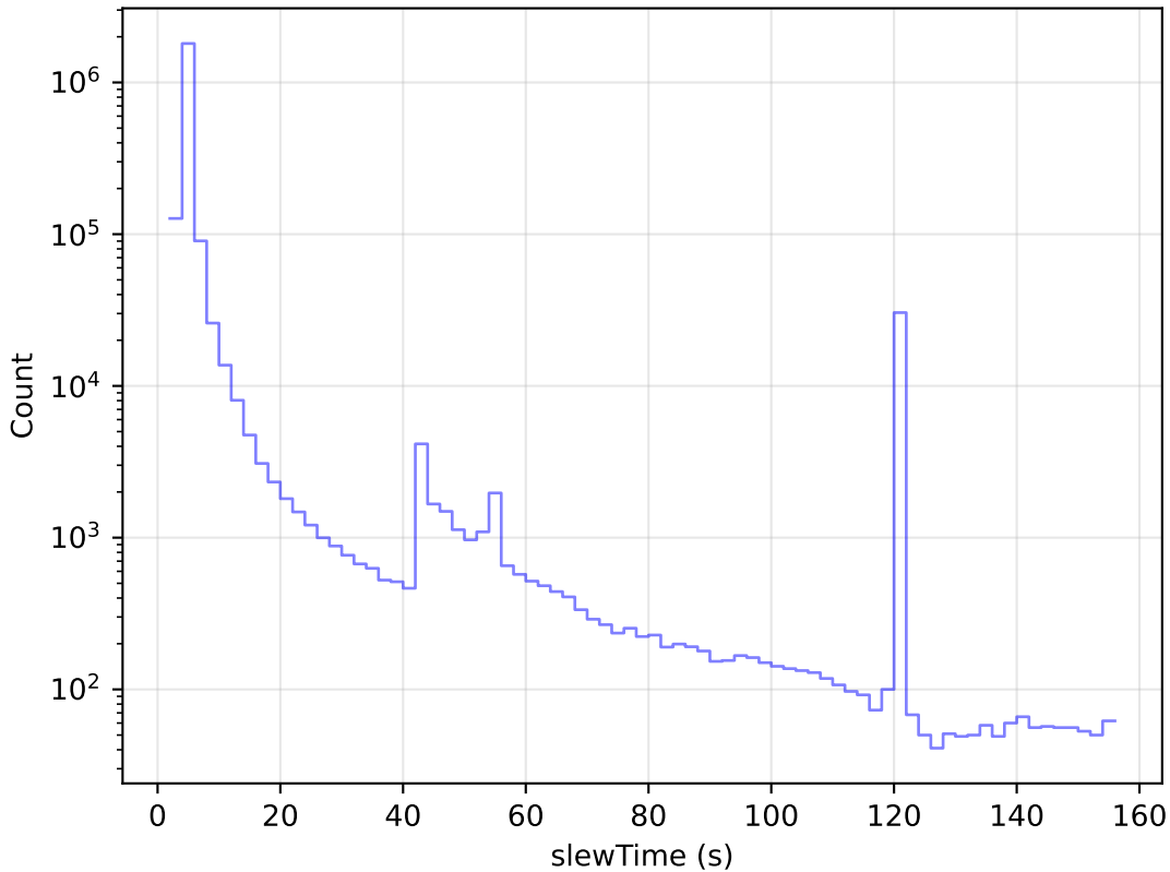
ddf_acor_sf25_lsf30_lsr20_v3.4_10yrs All visits: Slew Time Histogram
