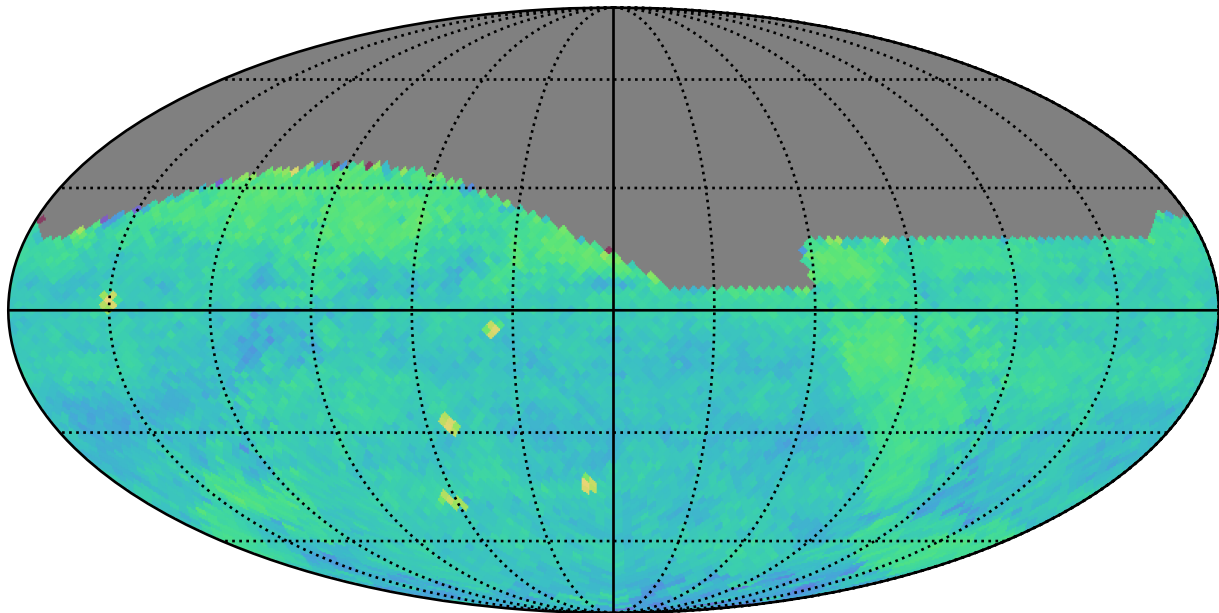
ddf_acor_sf25_lsf30_lsr20_v3.4_10yrs (g or r or i): PairFraction
