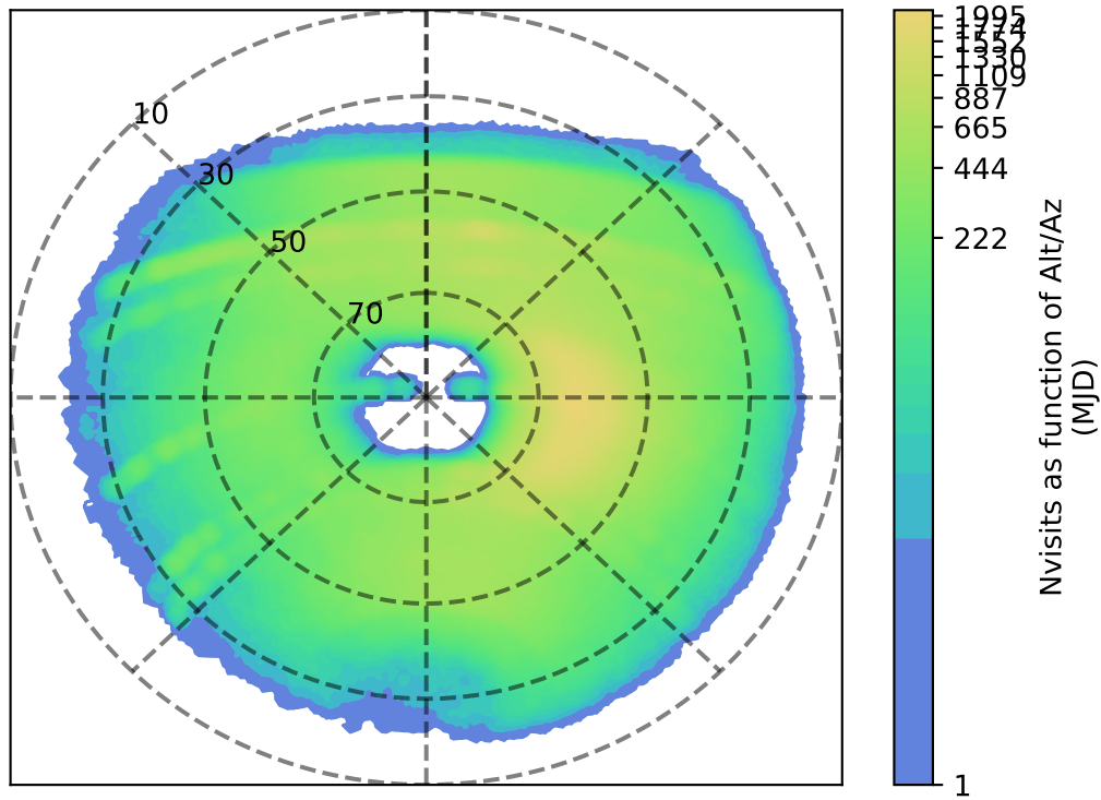
ddf_acor_sf25_lsf30_lsr20_v3.4_10yrs y: Nvisits as function of Alt/Az
